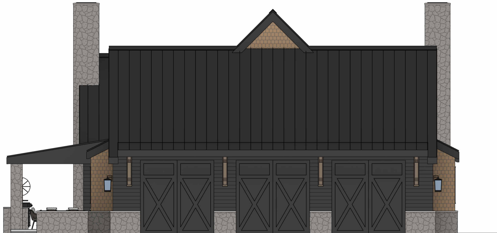
② WEST ELEVATION - PRESENTATION 1/8" = 1'-0"
