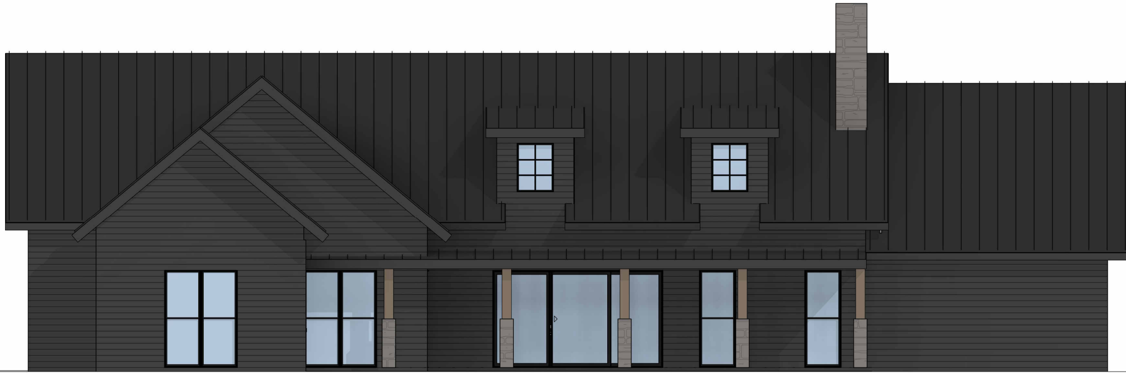
① NORTH ELEVATION - DESIGN 1/8" = 1'-0"
