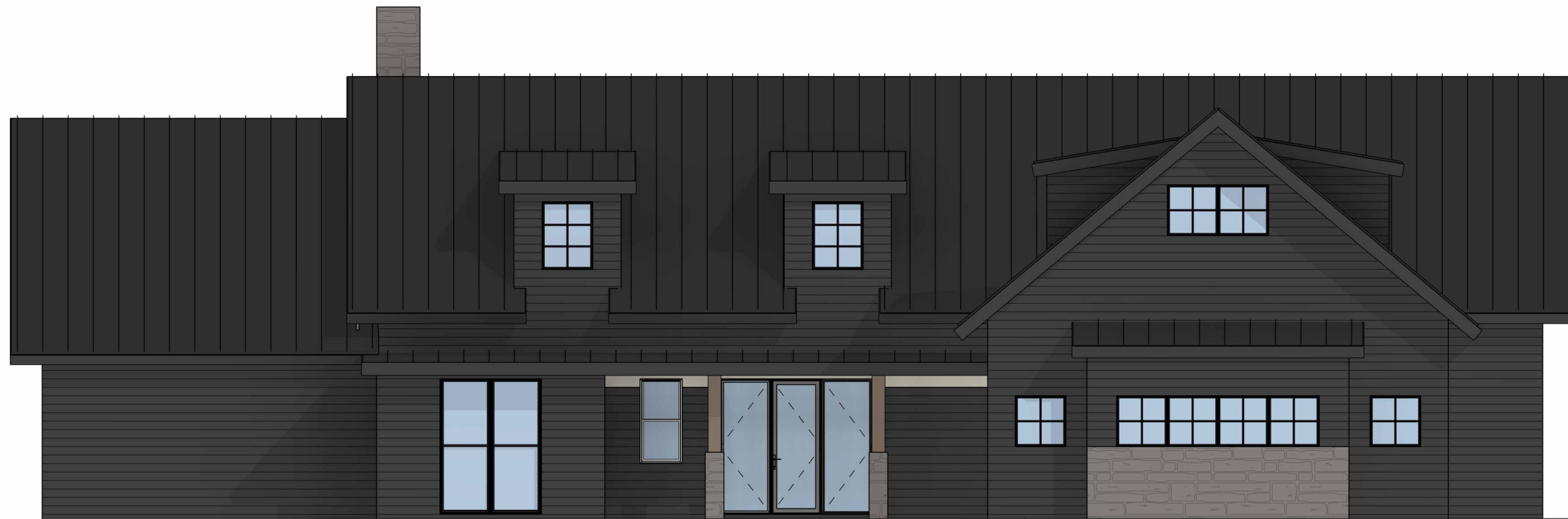
② SOUTH ELEVATION - DESIGN 1/8" = 1'-0"
