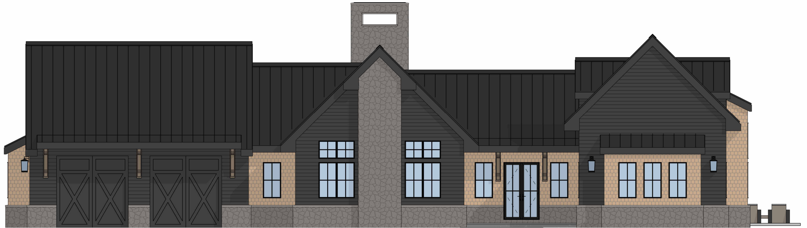
① SOUTH ELEVATION - PRESENTATION 1/8" = 1'-0"
